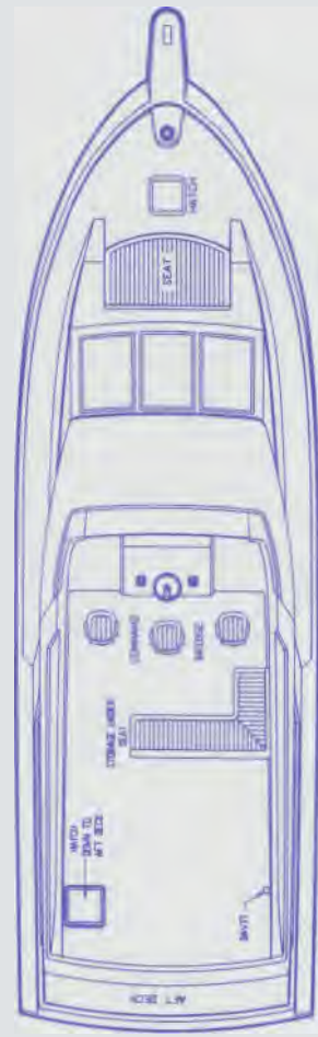
BRIDGE DECK
