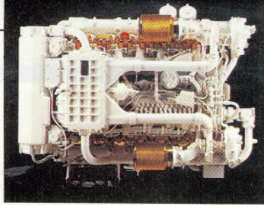
1100 HP 12-CYLINDER TURBOCHARGED, MAN 2842
