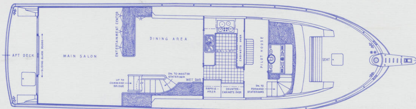
UPPER LEVEL
