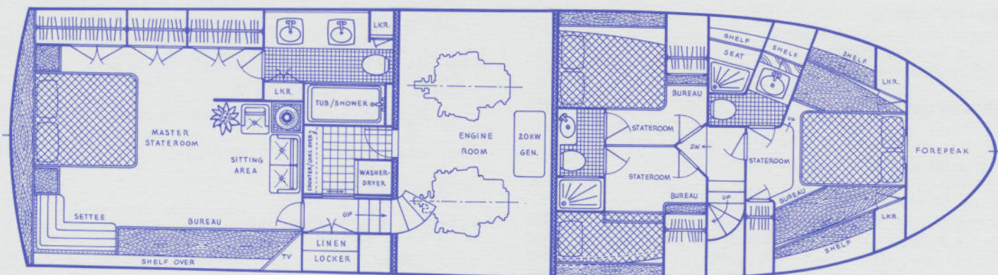
LOWER LEVEL
