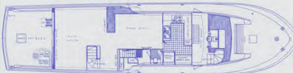
MAIN DECK
